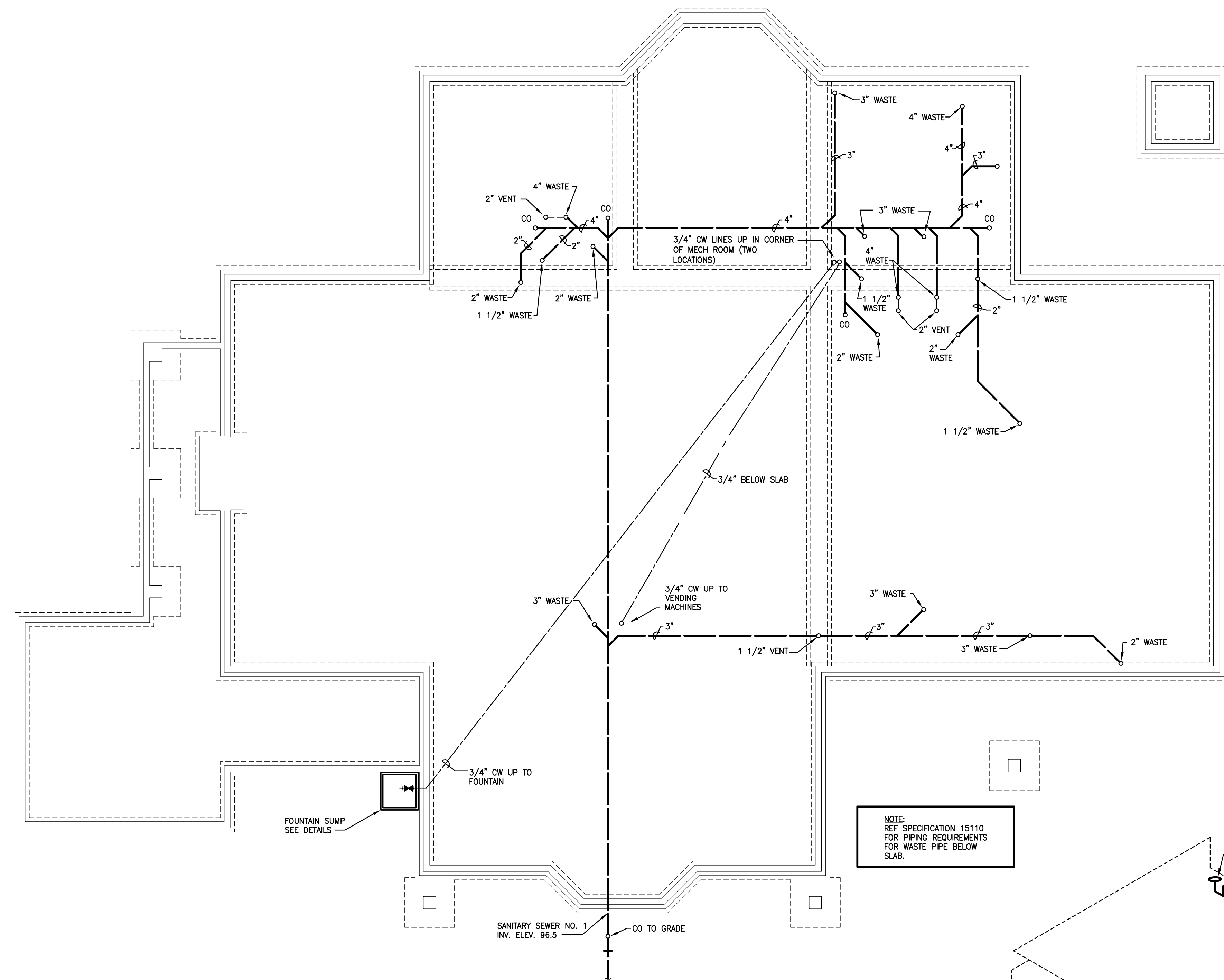
FOUNDATION PLUMBING PLAN SCALE: 3/16" = 1'-0"
